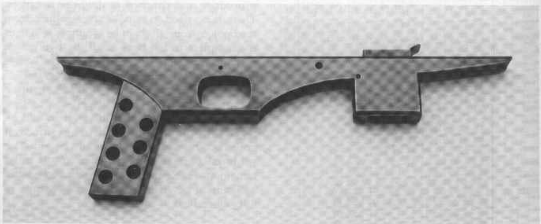
PHOTO 39: Side view of lower receiver with grip and well in position.
