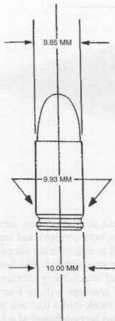
THIS CARTRIDGE CASE TAPERS FROM 9.93 MM TO 9.65 MM. THE BASE OF THE CASE IS 10 MM IN DIAMETER.
