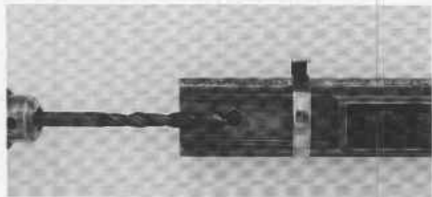
PHOTO 7: Drill through lower receiver bolt holes and into upper receiver tube.
