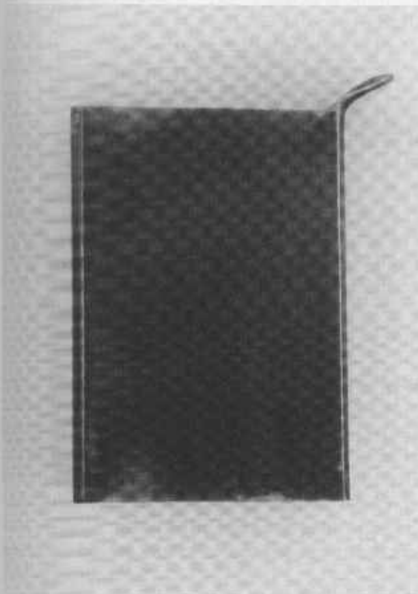
PHOTO 37: The magazine well with feed ramp bent to correct shape.
