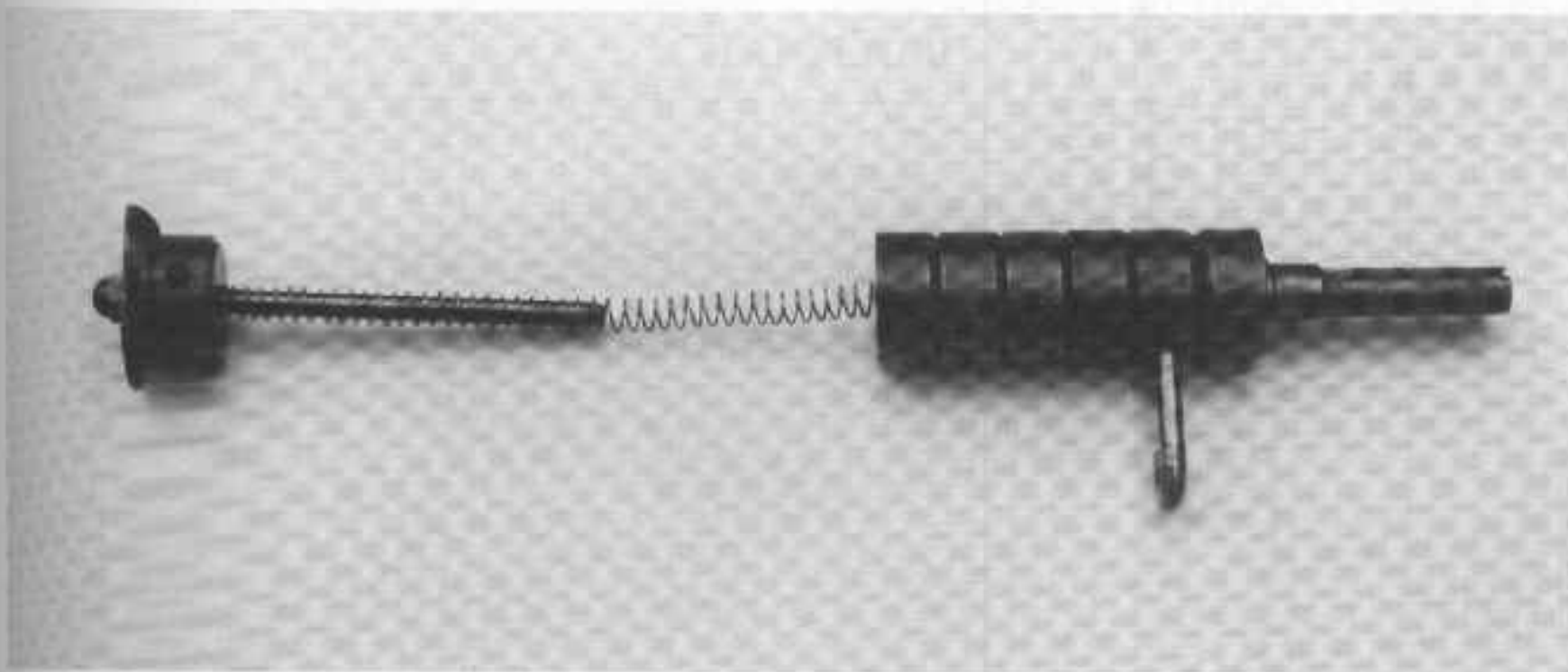
PHOTO 35: The recoil shield, guide, mainspring, and breech block shown in their respective positions.
