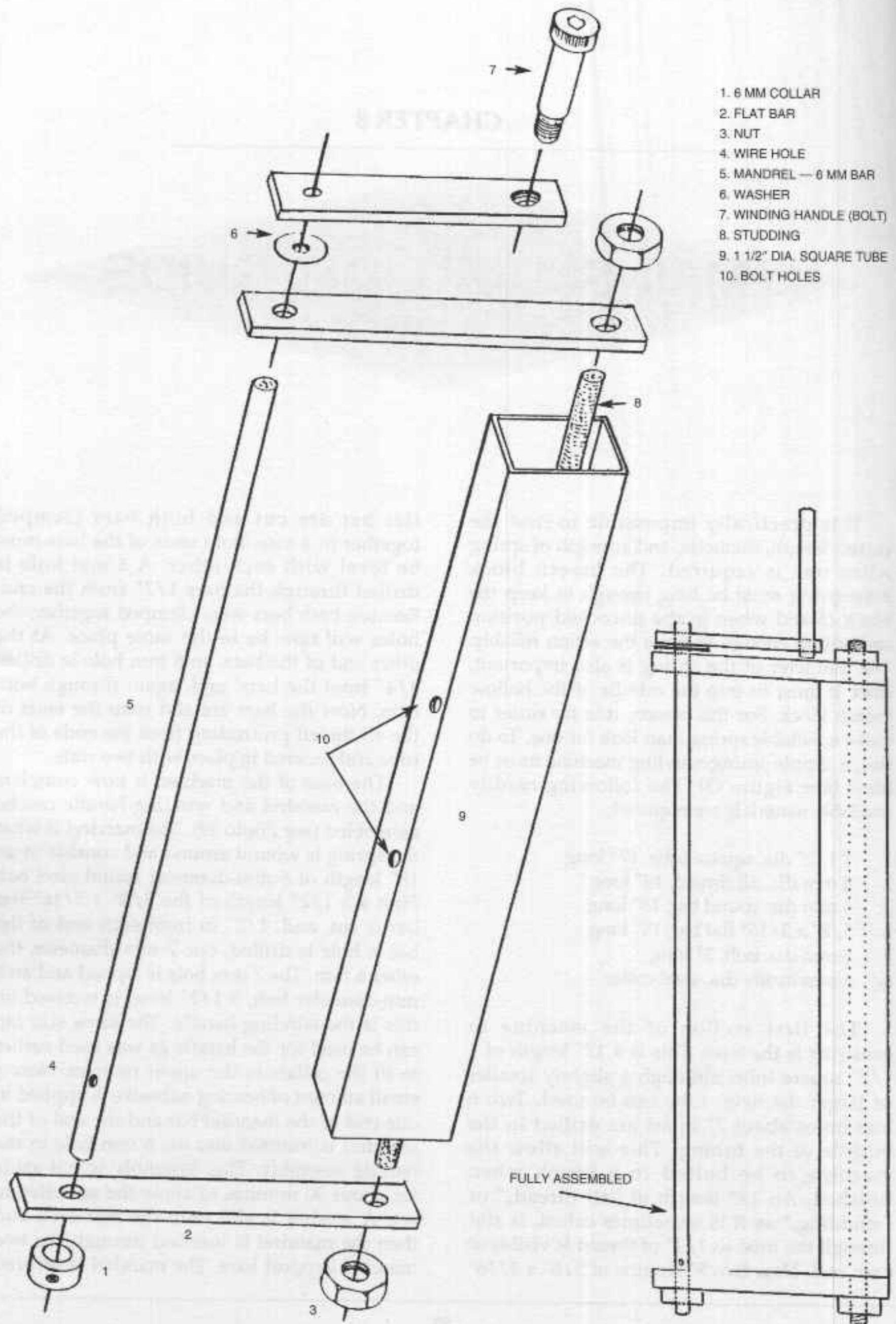
FIGURE O SPRING-WINDING MACHINE
